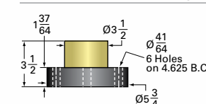
15-MSJ Acme Nut and Flange
