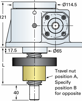
EM5-MSJ-IR INVERTED ROTATING For ordering, specify "L" dimension L(min) = travel + 103
