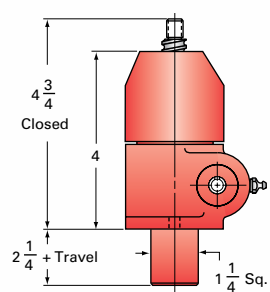
0.5-BSJ-IK & 0.5HL-BSJ-IK UPRIGHT KEYED
