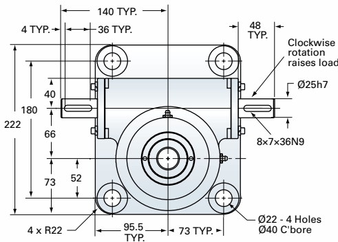
EM10-MSJ TOP VIEW
