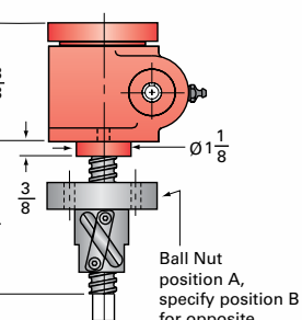
0.5-BSJ-IR & 0.5HL-BSJ-IR INVERTED ROTATING FOR ORDERING: Specify "L" dimension L (min) = Travel + 2 5/8
