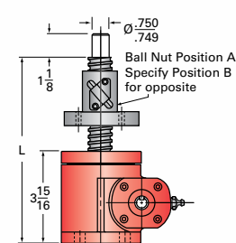
2-BSJ-UR UPRIGHT ROTATING
