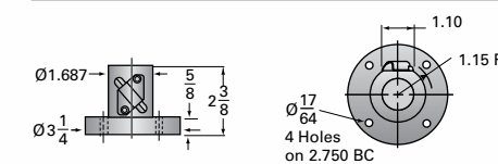
2-BSJ Ball Nut and Flange
