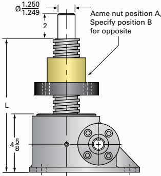
10SS-MSJ-UR UPRIGHT ROTATING For ordering, specify "L" dimension L(min) = travel + 8 5/8
