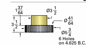
20-MSJ Acme Nut and Flange
