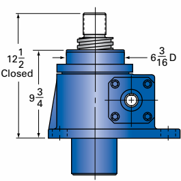
30-MSJ-UK UPRIGHT KEYED*
