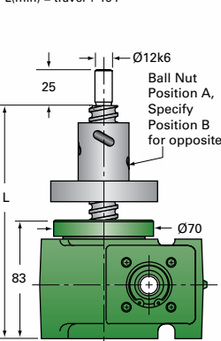
EM1-BSJ-UR UPRIGHT ROTATING For ordering, specify "L" dimension L(min) = travel + 164
