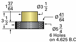
20SS-MSJ Acme Nut and Flange
