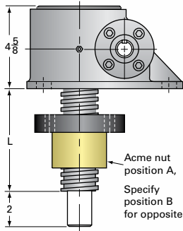
10SS-MSJ-IR INVERTED ROTATING For ordering, specify "L" dimension L(min) = travel + 4
