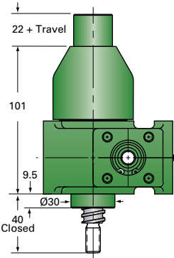
EM05-BSJ-I INVERTED
