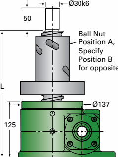
EM10-BSJ-UR UPRIGHT ROTATING For ordering, specify "L" dimension L(min) = travel + 283
