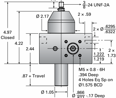
0.5C-BSJ-U &amp; 0.5CHL-BSJ-U UPRIGHT
