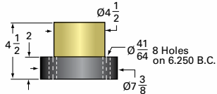
30-MSJ Acme Nut and Flange
