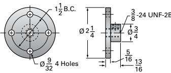
Top Plate (optional): 9000-EM-12
