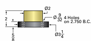
2.5-MSJ Acme Nut and Flange
