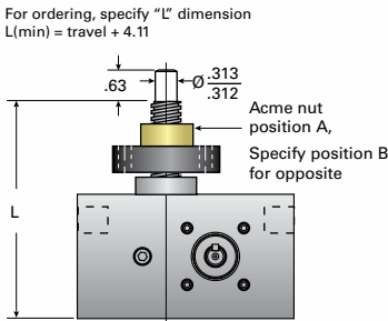
MJC-xx-UR UPRIGHT & INVERTED ROTATING
