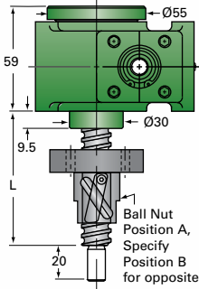
EM05-BSJ-IR INVERTED ROTATING
