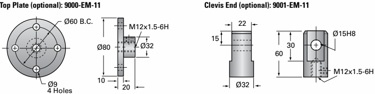
EM1C-MSJ Options (Standard Steel Parts)
