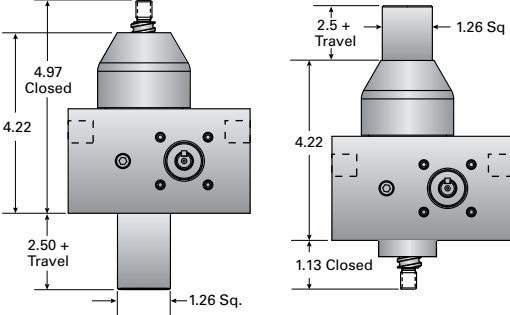
0.5C-BSJ-UK & 0.5CHL-BSJ-UK UPRIGHT KEYED 0.5C-BSJ-IK & 0.5CHL-BSJ-IK INVERTED KEYED
