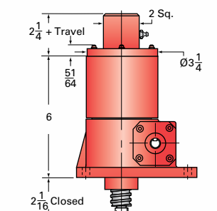
2.5HL-BSJ-1K INVERTED KEYED
