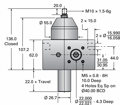
EM05C-BSJ-U UPRIGHT
