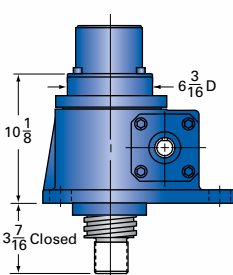
30-MSJ-IK INVERTED KEYED*
