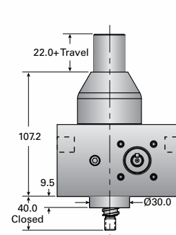
EM05C-BSJ-I INVERTED
