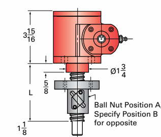
2-BSJ-IR INVERTED ROTATING
