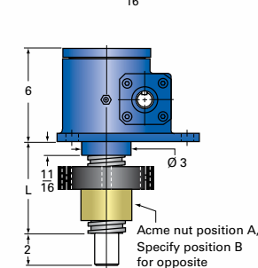
15-MSJ-IR INVERTED ROTATING
