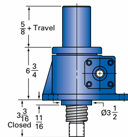
20-MSJ-I INVERTED
