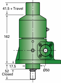
EM2.5-BSJ-I INVERTED
