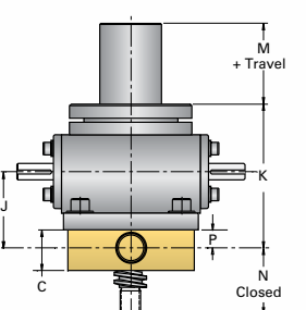
MSJ-I (Machine Screw Inverted)
