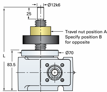
EM1-MSJ-UR UPRIGHT ROTATING
