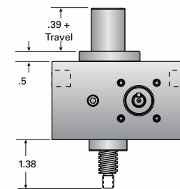
1ABC-MSJ-I INVERTED ANTI-BACKLASH
