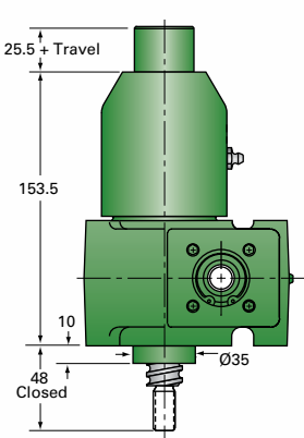
EM1-BSJ-I INVERTED
