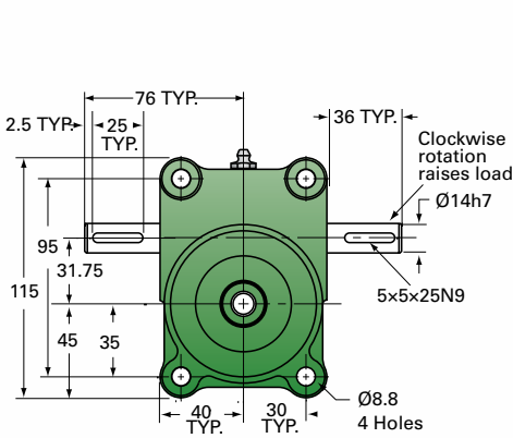
EM1-BSJ TOP VIEW
