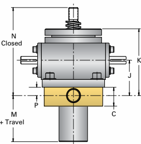
MSJ-U (Machine Screw Upright)
