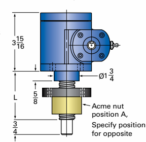
2-MSJ-IR INVERTED ROTATING
