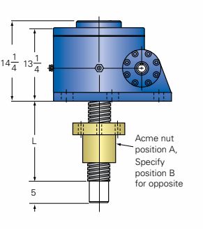
100-MSJ-IR INVERTED ROTATING
