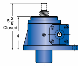
2.5AB-MSJ-U UPRIGHT ANTI-BACKLASH
