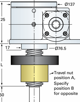
EM10-MSJ-IR INVERTED ROTATING
