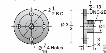
1C-BSJ & 1CHL Options (Standard Steel Parts)
