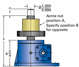
5-MSJ-UR UPRIGHT ROTATING
