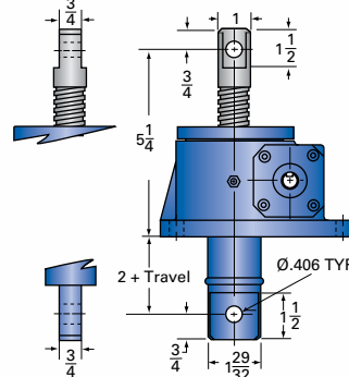
2.5-MSJ-DC DOUBLE CLEVIS
