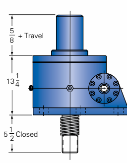
100-MSJ-I INVERTED
