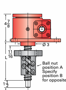
10-BSJ-IR & 10HL-BSJ-IR INVERTED ROTATING
