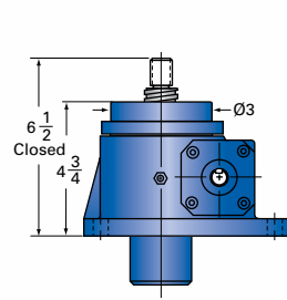
2.5-MSJ-UK UPRIGHT KEYED
