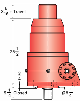
100-BSJ-I INVERTED
