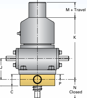
MSJ-I (Machine Screw Inverted)
