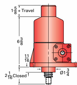
2.5HL-BSJ-I INVERTED
