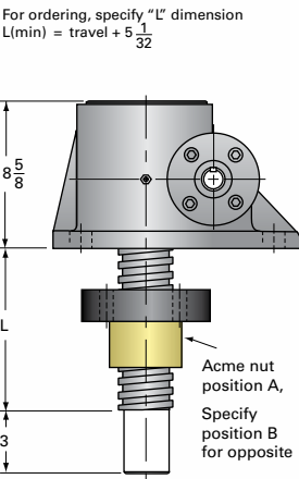
25SS-MSJ-IR INVERTED ROTATING
