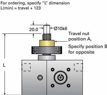
EM05C-MSJ-UR UPRIGHT & INVERTED ROTATING
