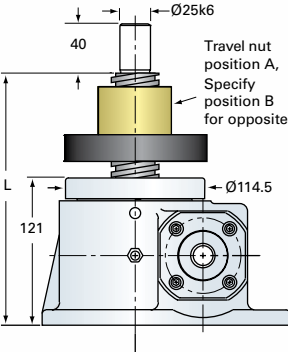
EM5-MSJ-UR UPRIGHT ROTATING For ordering, specify "L" dimension L(min) = travel + 207
