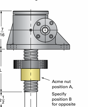
20SS-MSJ-IR INVERTED ROTATING
