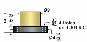
5-MSJ Acme Nut and Flange
