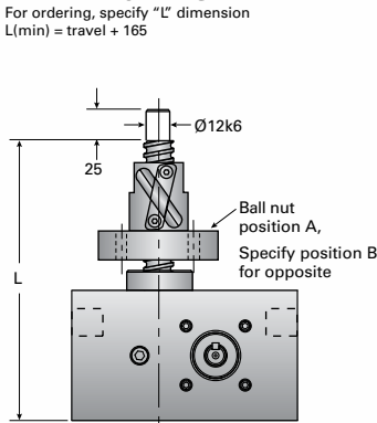
EM1C-BSJ-UR UPRIGHT & INVERTED ROTATING
