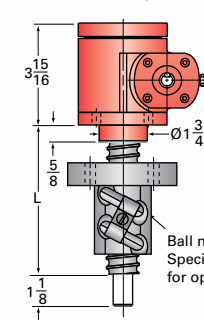
3-BSJ-IR INVERTED ROTATING
