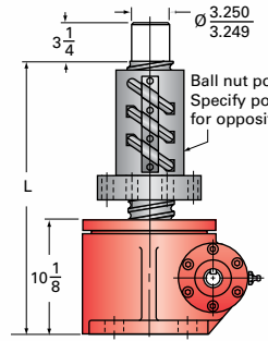
50-BSJ-UR UPRIGHT ROTATING
