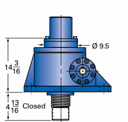
75-MSJ-IK INVERTED KEYED*
