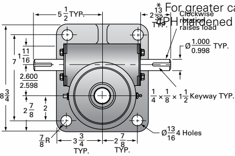
10SS-MSJ TOP VIEW
