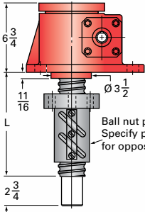
20-BSJ-IR & 20HL-BSJ-IR INVERTED ROTATING For ordering, specify "L" dimension L(min) = travel + 8 7/16
