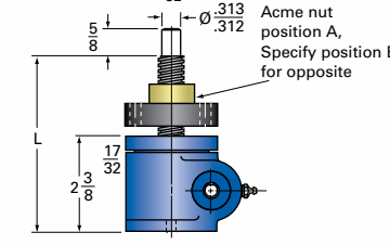
MJ-xx-UR UPRIGHT ROTATING
