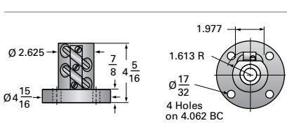
10-BSJ Ball Nut and Flange
