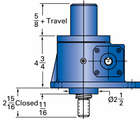
5-MSJ-I INVERTED
