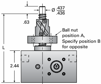
0.5C-BSJ-UR & 0.5CHL-BSJ-UR UPRIGHT or INVERTED ROTATING FOR ORDERING: Specify "L" dimension L (min) = Travel + 5.08
