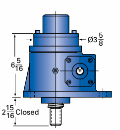
5-MSJ-IK INVERTED KEYED
