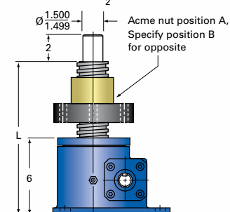
15-MSJ-UR UPRIGHT ROTATING
