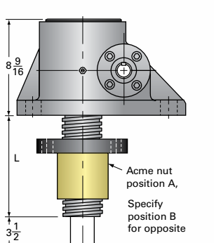
35SS-MSJ-IR INVERTED ROTATING
