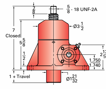
2R-BSJ-U UPRIGHT
