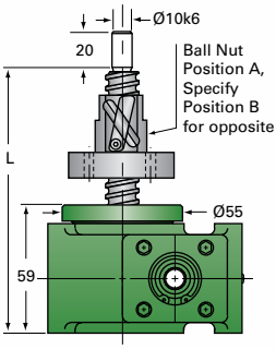
EM05-BSJ-UR UPRIGHT ROTATING
