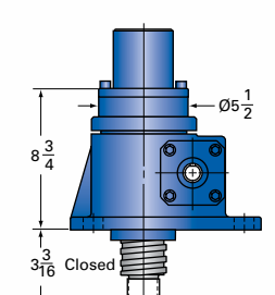
20-MSJ-1K INVERTED KEYED
