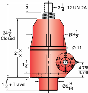
50-BSJ-U UPRIGHT
