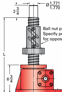
20-BSJ-UR & 20HL-BSJ-UR UPRIGHT ROTATING For ordering, specify "L" dimension L(min) = travel + 14 1/2
