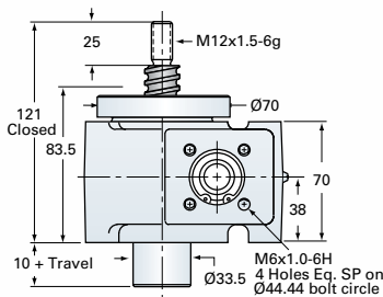
EM1-MSJ-U UPRIGHT
