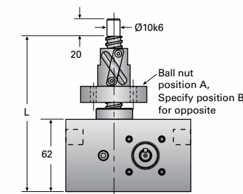
EM05C-BSJ-UR UPRIGHT & INVERTED ROTATING
