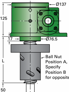
EM10-BSJ-IR INVERTED ROTATING For ordering, specify "L" dimension L(min) = travel + 173
