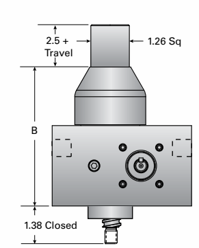
1C-BSJ-IK & 1CHL-BSJ-IK INVERTED KEYED
