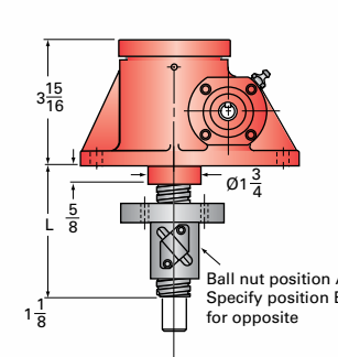
2R-BSJ-IR INVERTED ROTATING
