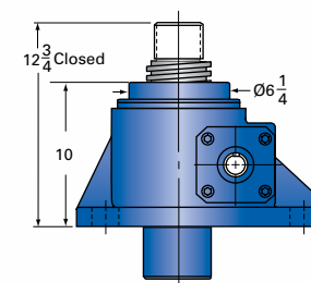
35-MSJ-UK UPRIGHT KEYED*
