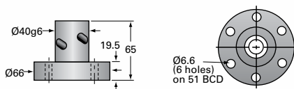
EM2.5-BSJ Ball Nut and Flange
