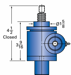
1-MSJ-UK UPRIGHT KEYED
