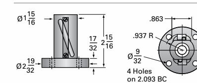
1CHL-BSJ Ball Nut and Flange
