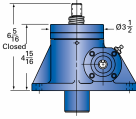
2R-MSJ-UK UPRIGHT KEYED
