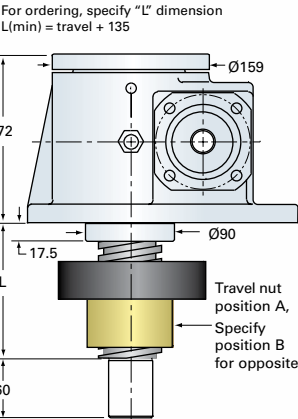
EM20-MSJ-IR INVERTED ROTATING
