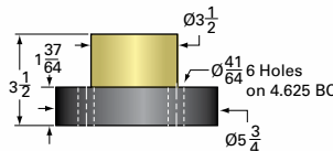
15SS-MSJ Acme Nut and Flange
