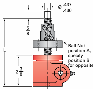
0.5-BSJ-UR & 0.5HL-BSJ-UR UPRIGHT ROTATING FOR ORDERING: Specify "L" dimension L (min) = Travel + 4 3/8
