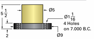
35SS-MSJ Acme Nut and Flange
