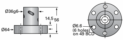
EM1C-BSJ Ball Nut and Flange
