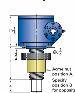
50-MSJ-IR INVERTED ROTATING
