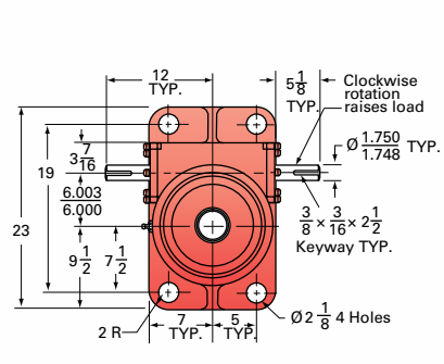
75-BSJ TOP VIEW
