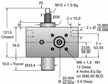
EM1C-MSJ-U UPRIGHT & INVERTED
