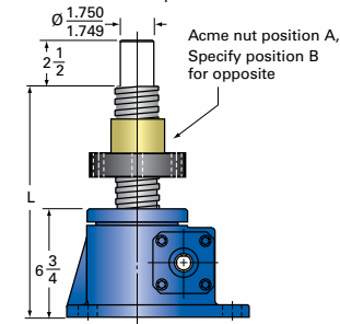
20-MSJ-UR UPRIGHT ROTATING For ordering, specify "L" dimension.
