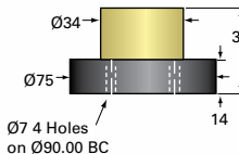
EM1-MSJ Travel Nut and Flange
