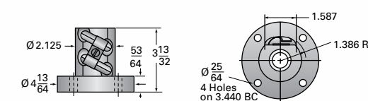
3-BSJ Ball Nut and Flange
