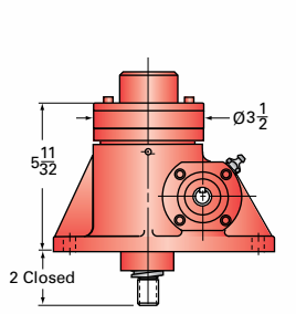
2R-BSJ-1K INVERTED KEYED
