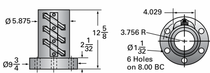
100-BSJ Ball Nut and Flange
