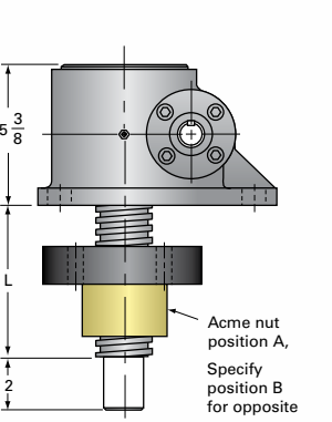
15SS-MSJ-IR INVERTED ROTATING
