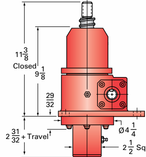
10-BSJ-IK & 10HL-BSJ-IK UPRIGHT KEYED
