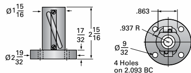
1HL-BSJ Ball Nut and Flange
