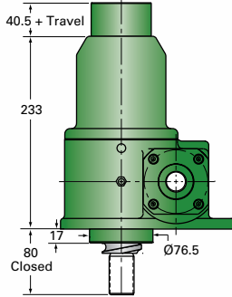
EM10-BSJ-I INVERTED
