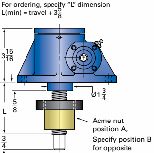
2R-MSJ-IR INVERTED ROTATING
