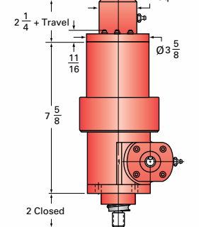
3-BSJ-1K INVERTED KEYED
