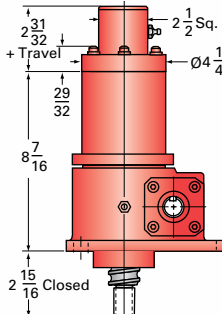
10-BSJ-IK & 10HL-BSJ-IK INVERTED KEYED
