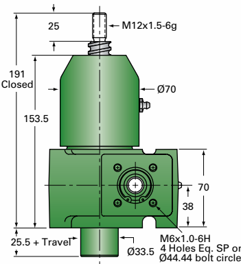
EM1-BSJ-U UPRIGHT
