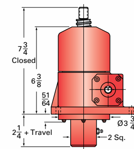
2.5HL-BSJ-UK UPRIGHT KEYED
