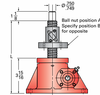
2R-BSJ-UR UPRIGHT ROTATING
