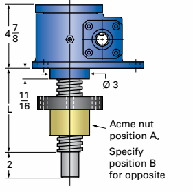
10-MSJ-IR INVERTED ROTATING
