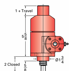
2-BSJ-I INVERTED
