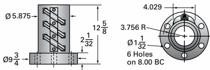
50-BSJ Ball Nut and Flange
