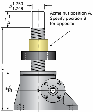
20SS-MSJ-UR UPRIGHT ROTATING
