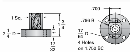
0.5HL-BSJ Ball Nut and Flange
