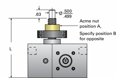
1C-MSJ-UR UPRIGHT & INVERTED ROTATING
