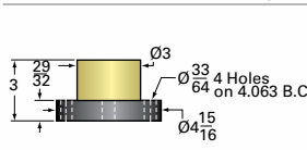
10-MSJ Acme Nut and Flange
