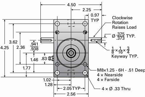
MJC-xx TOP VIEW
