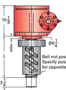
50-BSJ-IR INVERTED ROTATING
