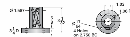
2.5HL-BSJ Ball Nut and Flange
