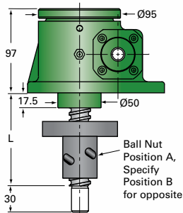
EM2.5-BSJ-IR INVERTED ROTATING For ordering, specify "L" dimension L(min) = travel + 107
