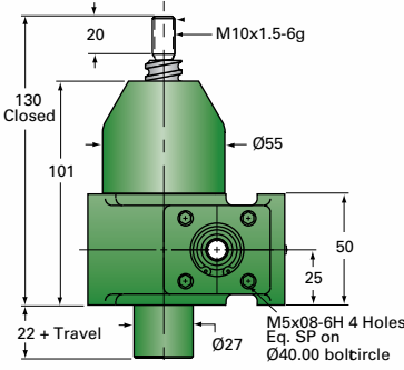
EM05-BSJ-U UPRIGHT
