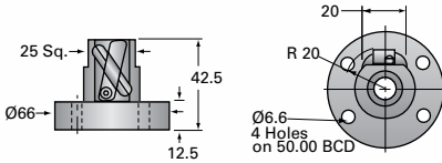
EM05-BSJ Ball Nut and Flange
