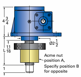
5-MSJ-IR INVERTED ROTATING
