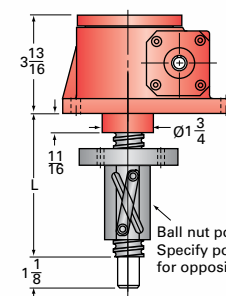
2.5HL-BSJ-IR INVERTED ROTATING
