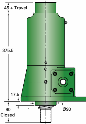
EM20-BSJ-I INVERTED
