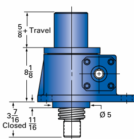
30-MSJ-I INVERTED
