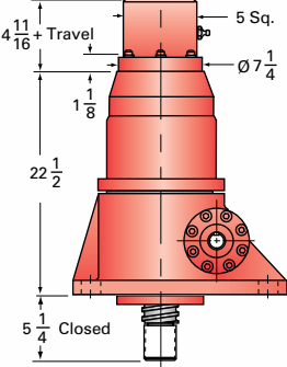
75-BSJ- I INVERTED KEYED
