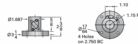
2.5-BSJ Ball Nut and Flange
