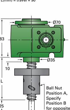
EM1-BSJ-IR INVERTED ROTATING For ordering, specify "L" dimension L(min) = travel + 90
