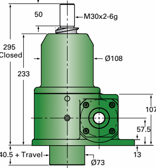
EM10-BSJ-U UPRIGHT
