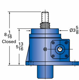
5-MSJ-UK UPRIGHT KEYED
