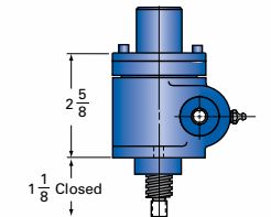
MJ-xx-IK INVERTED KEYED
