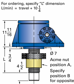
75-MSJ-IR INVERTED ROTATING
