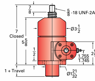
2-BSJ-U UPRIGHT
