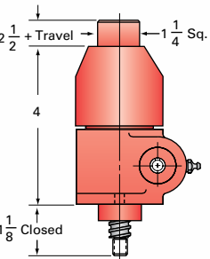
0.5-BSJ-IK & 0.5HL-BSJ-IK INVERTED KEYED
