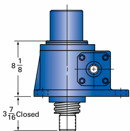
30AB-MSJ-I INVERTED ANTI-BACKLASH
