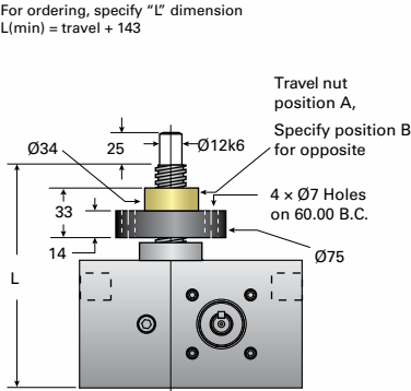
EM1C-MSJ-UR UPRIGHT & INVERTED ROTATING
