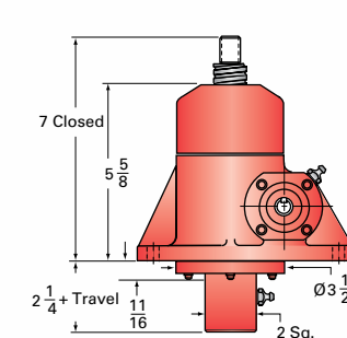
2R-BSJ-UK UPRIGHT KEYED
