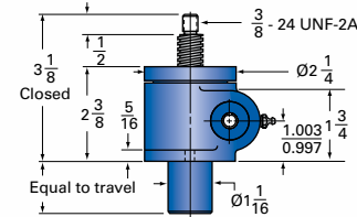
MJ-xx-U UPRIGHT
