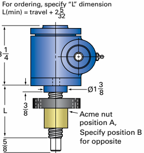
1-MSJ-IR INVERTED ROTATING
