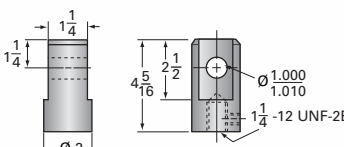
Clevis End (optional): 9001-SS-03
