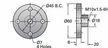
Motor Mounts
