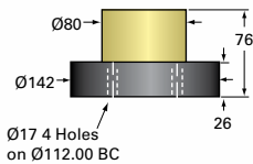
EM10-MSJ Travel Nut and Flange
