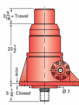
75-BSJ-I INVERTED
