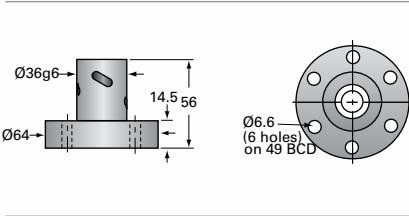
EM1-BSJ Ball Nut and Flange
