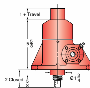
2R-BSJ-I INVERTED
