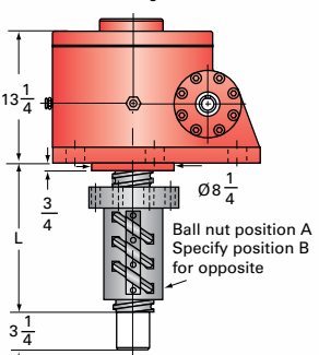
100-BSJ-IR INVERTED ROTATING
