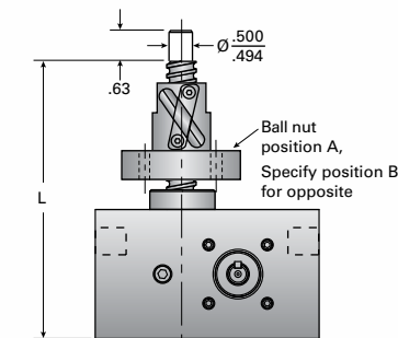
1C-BSJ-UR & 1CHL-BSJ-UR UPRIGHT & INVERTED ROTATING
