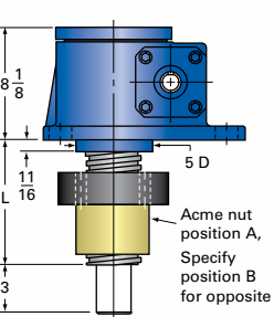
30-MSJ-IR INVERTED ROTATING
