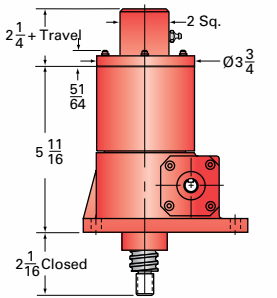
2.5-BSJ-IK INVERTED KEYED
