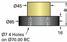
EM2.5-MSJ Travel Nut and Flange
