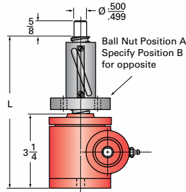
1HL-BSJ-UR UPRIGHT ROTATING
