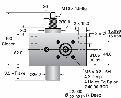
EM05C-MSJ-U UPRIGHT & INVERTED
