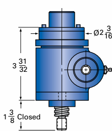
1-MSJ-IK INVERTED KEYED
