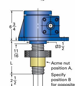
20-MSJ-IR INVERTED ROTATING
