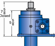
10AB-MSJ-U UPRIGHT ANTI-BACKLASH
