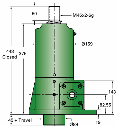
EM20-BSJ-U UPRIGHT
