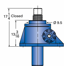
75-MSJ-UK UPRIGHT KEYED*
