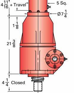
50-BSJ-IK INVERTED KEYED
