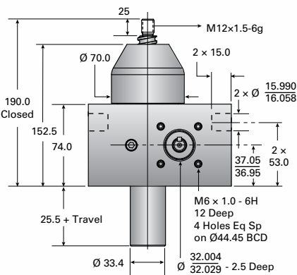
EM1C-BSJ-U UPRIGHT
