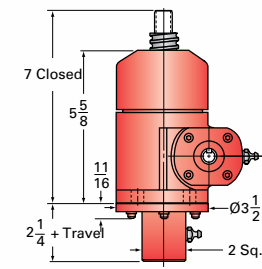
2-BSJ-UK UPRIGHT KEYED
