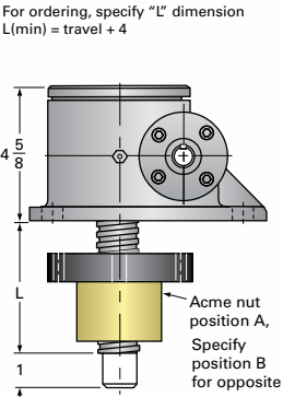
5SS-MSJ-IR INVERTED ROTATING
