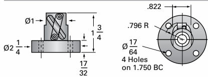
0.5CHL-BSJ Ball Nut and Flange
