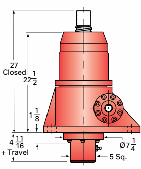
75-BSJ-UK UPRIGHT KEYED
