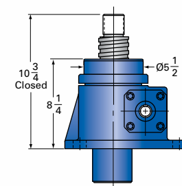
20-MSJ-UK UPRIGHT KEYED
