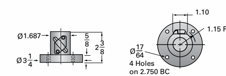
2R-BSJ Ball Nut and Flange
