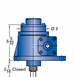
2.5-MSJ-IK INVERTED KEYED
