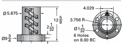
75-BSJ Ball Nut and Flange
