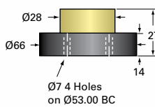
EM05-MSJ Nut and Flange
