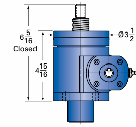
2-MSJ-UK UPRIGHT KEYED
