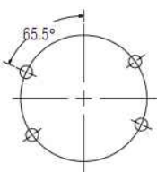
Coolant Inlet Port 8WCB
