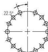
Coolant Inlet Port 36WCS
