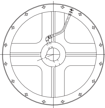
Single Connection
