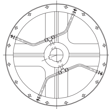
Four Connections
