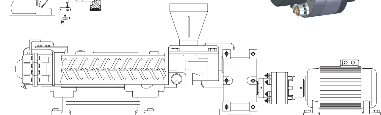
DSM torque limiter with coupling between motor and gearbox for extruder application
