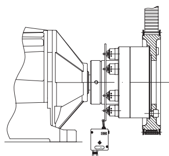
DSM/SI model with toothed pulley, complete with intervention signaling ring and electromechanical switch EM1.
