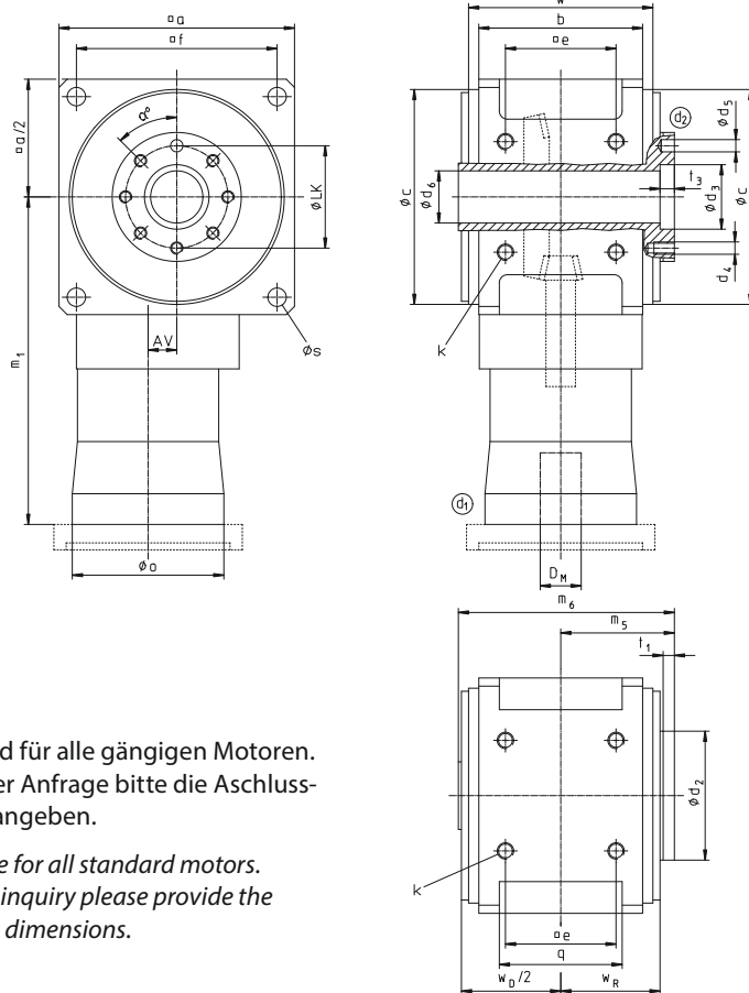
Abmessungen [mm] / dimensions [mm]
